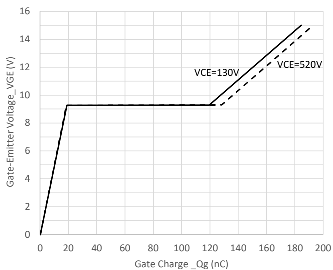
Gate Charge
