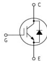
Built-in FRD
