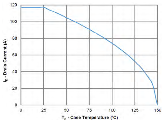
Figure 11: Current Derating
