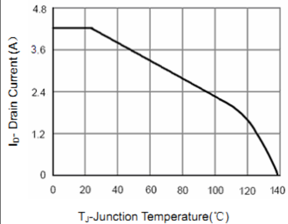
Figure 4 Drain Current
