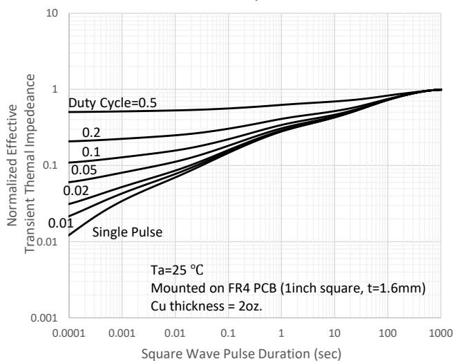
Thermal Response
