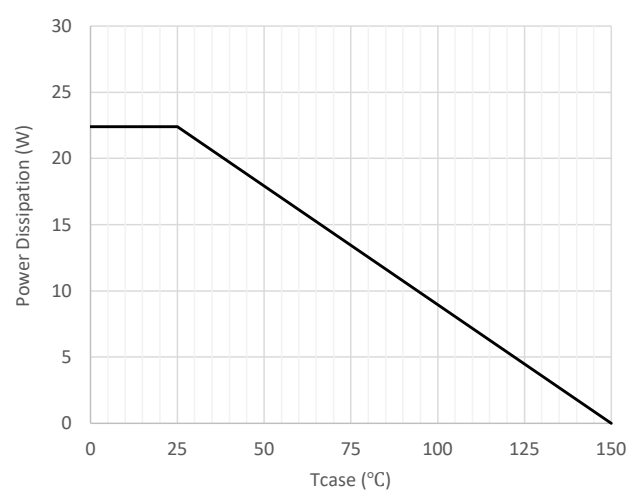
Power Derating
