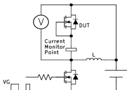
Test Circuit 9 trr/Qrr
