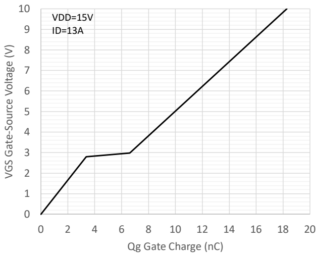
Gate-Charge Characteristics
